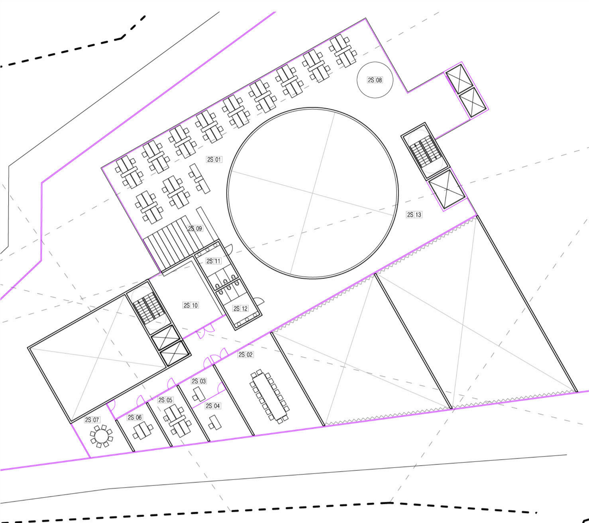
2ND FLOOR 1:250
